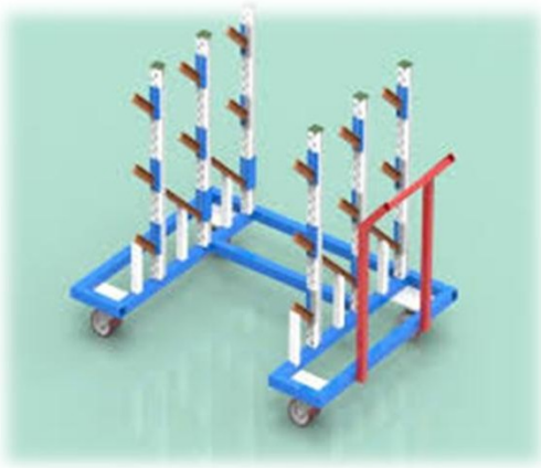
Child Parts Trolley
