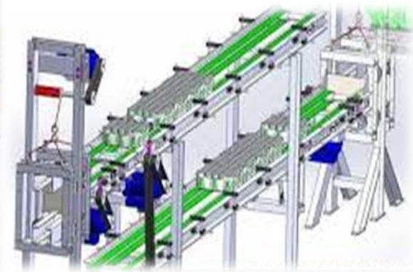
Double Belt Conveyors concept
