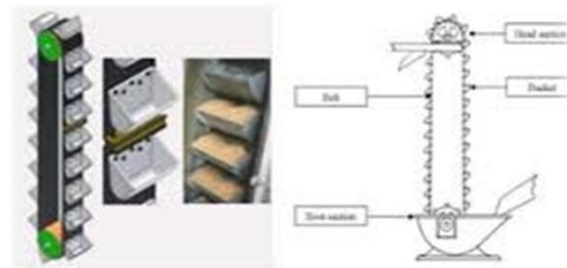
Bucket Elevator
